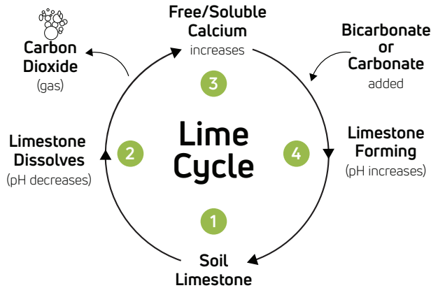
Figure 1. Lime Cycle
